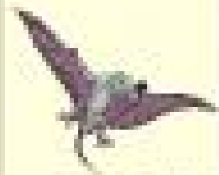
Pterosaur
