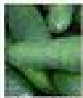
CUCUMBERS
