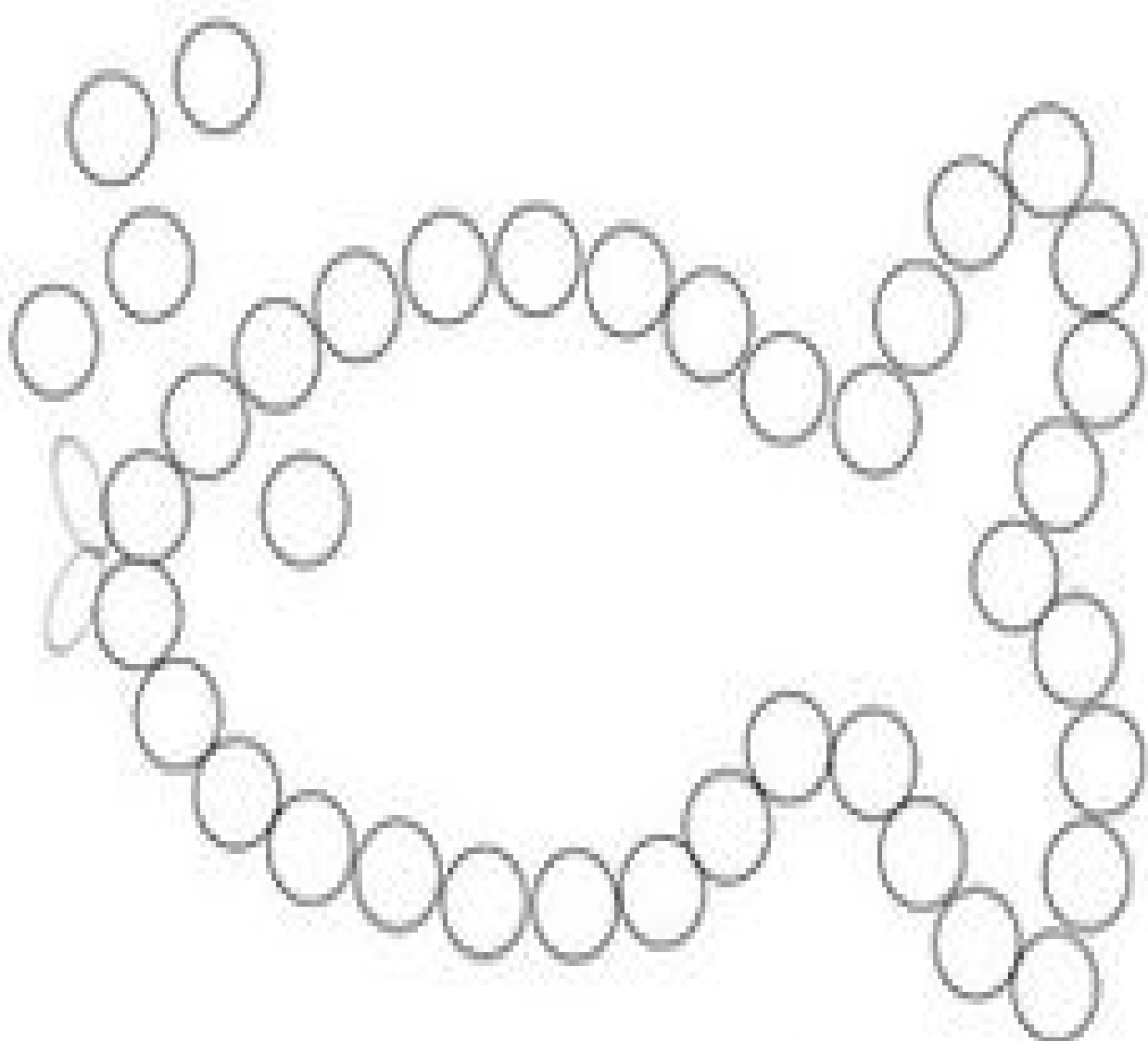
Fig. 1. The configuration of a ring of particles.
