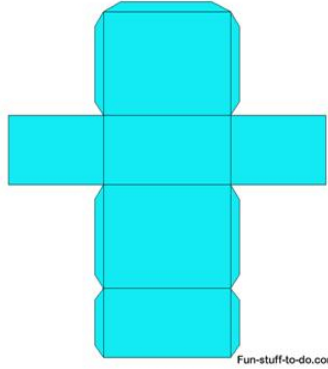
Rectangular Prism
