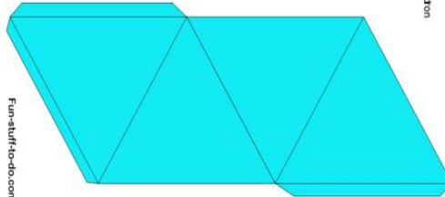
Tetrahedron
