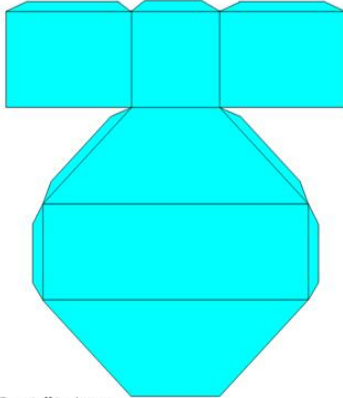
Trapezoidal Prism
