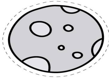
Mercury
