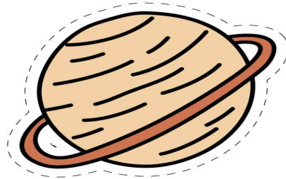
Saturn
