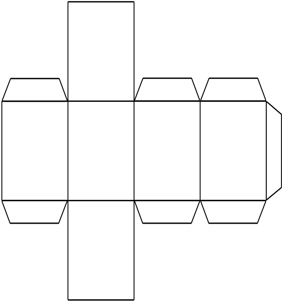
Hexahedron (platonic solid)
