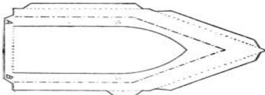
2. Plan of end of south aisle : half-scale Use scale-rule B
