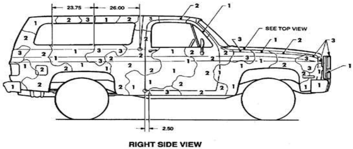
Figure 44a. Truck, utility: 3/4-ton, 4 x 4, M1009. (1 of 2) (complete repaint)
