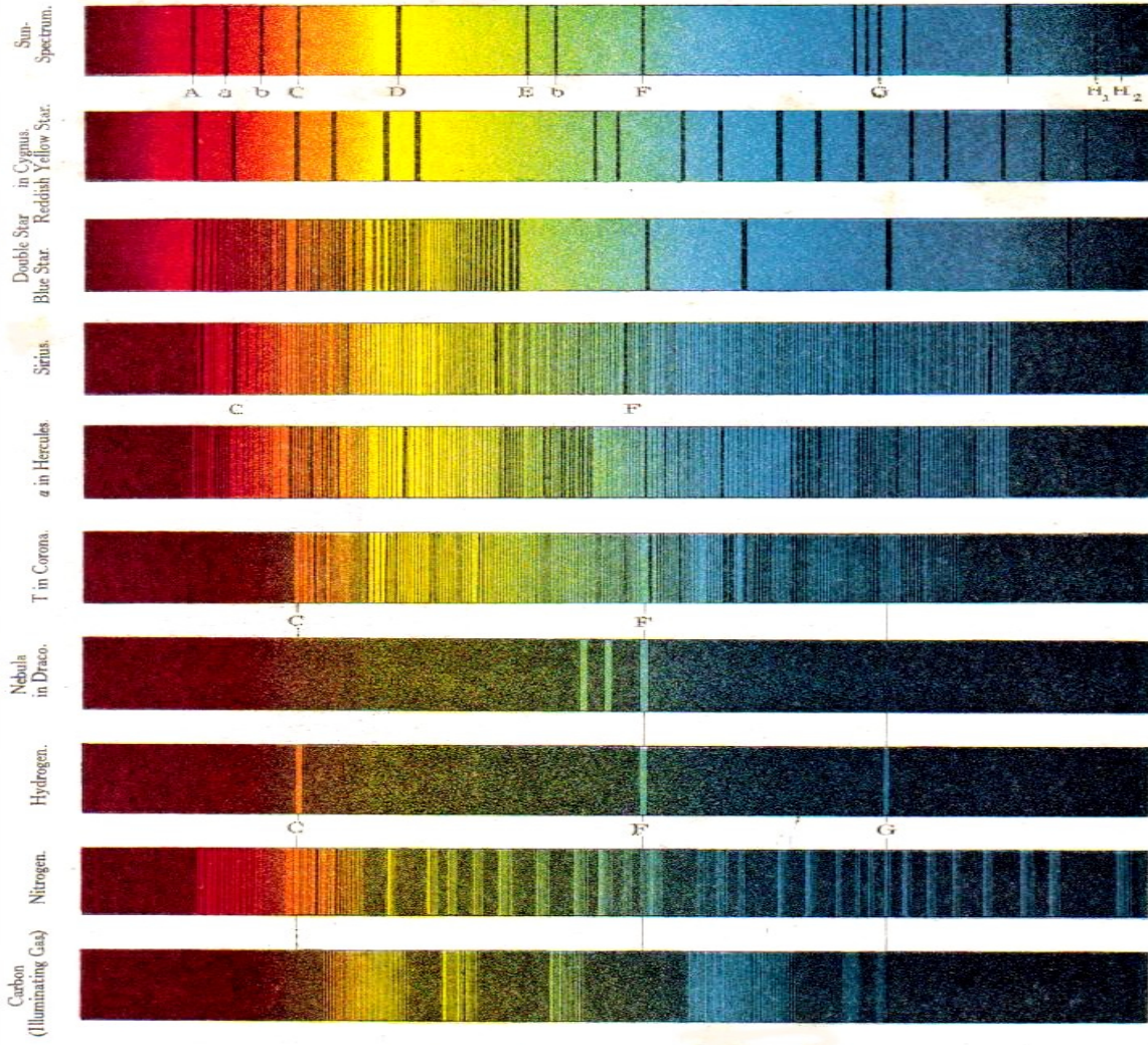
SPECTRA OF THE FIXED STARS AND NEBULAE COMPARED WITH THE SUN-SPECTRUM AND OTHER SPECTRA.
